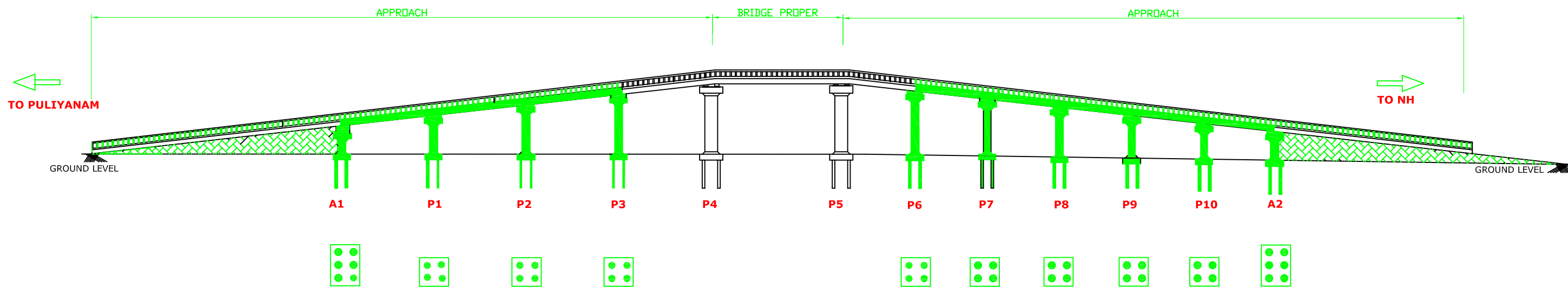
PILE FOUNDATION
